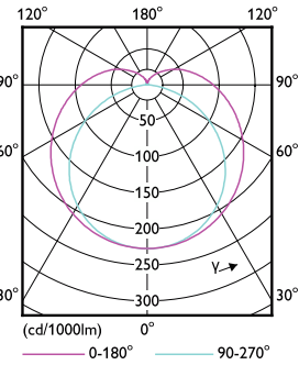
Light Distribution Diagram - MAS LEDtube 1200mm UO 13.5W 840 T8 EELB
