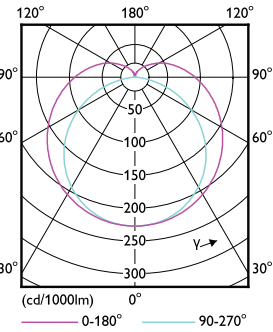
Light Distribution Diagram - MAS LEDtube 1200mm HO 11.3W 840 T8 EELB
