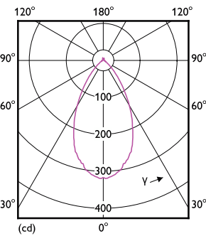
Light Distribution Diagram - MAS LED spot VLE D 3.7-50W GU10 927 60D
