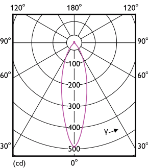
Light Distribution Diagram - MAS LED spot VLE D 2.8-35W GU10 940 36D
