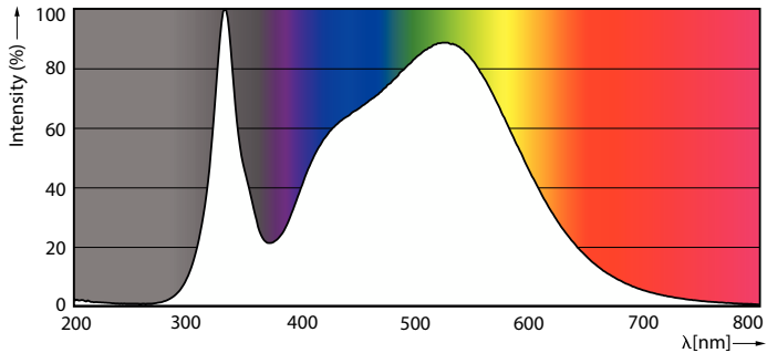
Spectral Power Distribution Colour - CorePro LEDtube 1200mm UO 17.7W 840 T8
