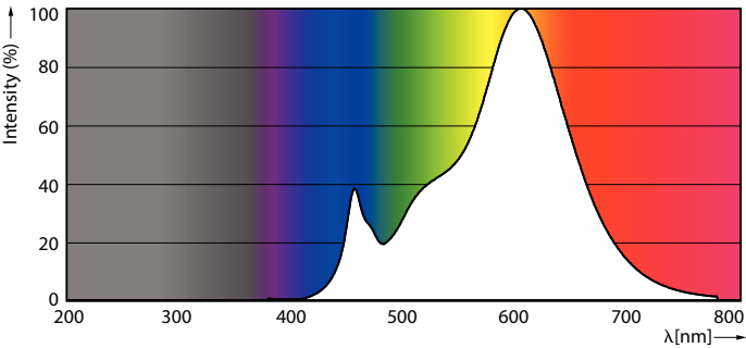
Spectral Power Distribution Colour - CorePro LEDcapsule 3.7-40W ND G9 827
