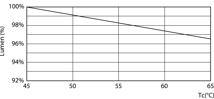
Lumen Maintenance Diagram - MAS LEDtube 900mm HE 11.5W 865 T5 EU
