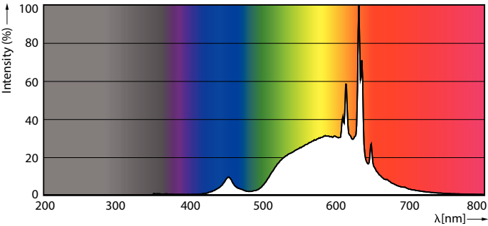
Spectral Power Distribution Colour - MAS LEDBulbND2.3-40W E27 827 A60 CL G UE
