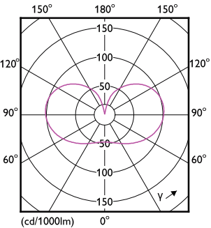
Light Distribution Diagram - MAS LEDBulb D 4-60W E27 830 A60 FR G UE
