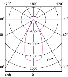
Light Distribution Diagram - MAS LEDExpertColor 20-100W 927 AR111 45D
