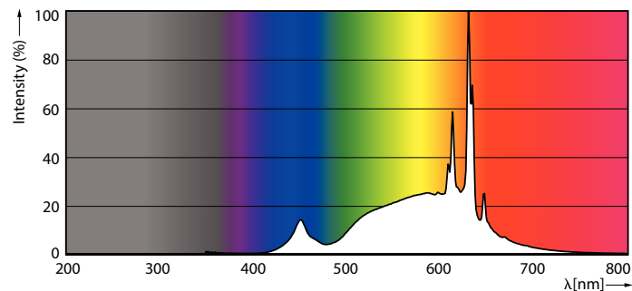
Spectral Power Distribution Colour - MAS VLE LEDLusterD3.4-40W E14 P45 927CLG
