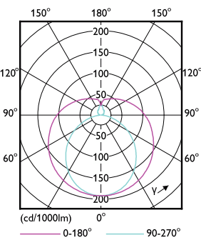
Light Distribution Diagram - MAS LEDtube VLE UN 1200mm UO 15.5W865 T8
