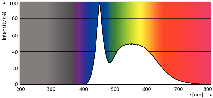
Spectral Power Distribution Colour - CorePro candle ND 5-40W E14 865 B35 FR
