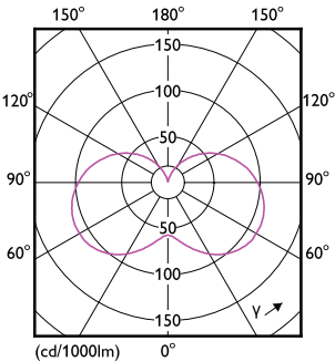
Light Distribution Diagram - CorePro candle ND 5-40W E14 840 B35 FR
