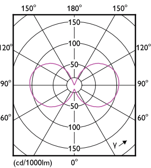
Light Distribution Diagram - CorePro LEDCandleND6.5-60W B35 E14840CLG
