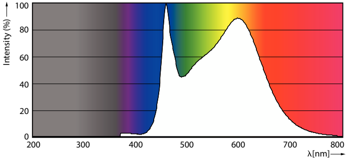
Spectral Power Distribution Colour - CorePro LEDCandleND4.3-40W E14 840B35CLG
