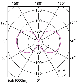
Light Distribution Diagram - CorePro LEDCandleND4.3-40W E14 840B35CLG
