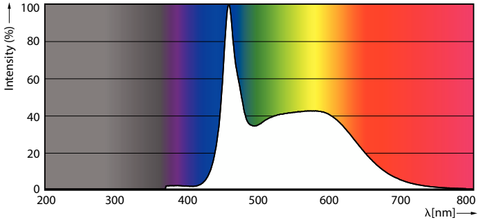
Spectral Power Distribution Colour - CorePro LEDBulbND 150W E27 A67 865 FR G
