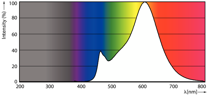
Spectral Power Distribution Colour - CorePro LEDBulbND 120W E27 A67 827 CL G
