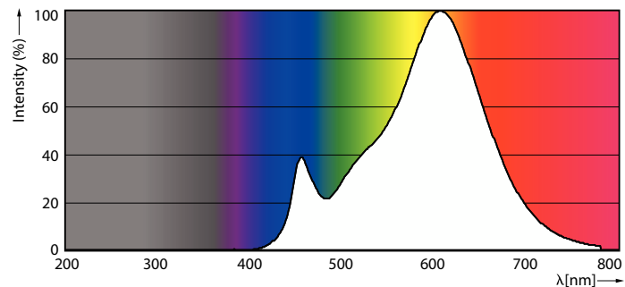
Spectral Power Distribution Colour - CorePro LED spot 2.3-20W 827 MR11 36D
